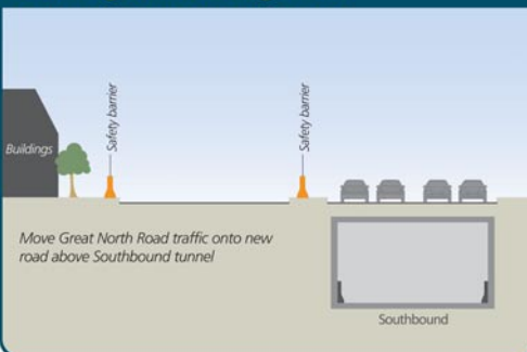
Installing traffic management
