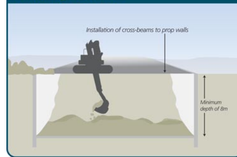
Excavating the tunnel
